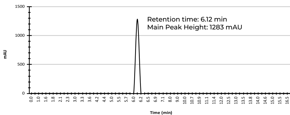
HPLC Chromatogram
