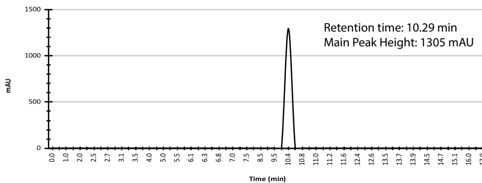
HPLC Chromatogram
