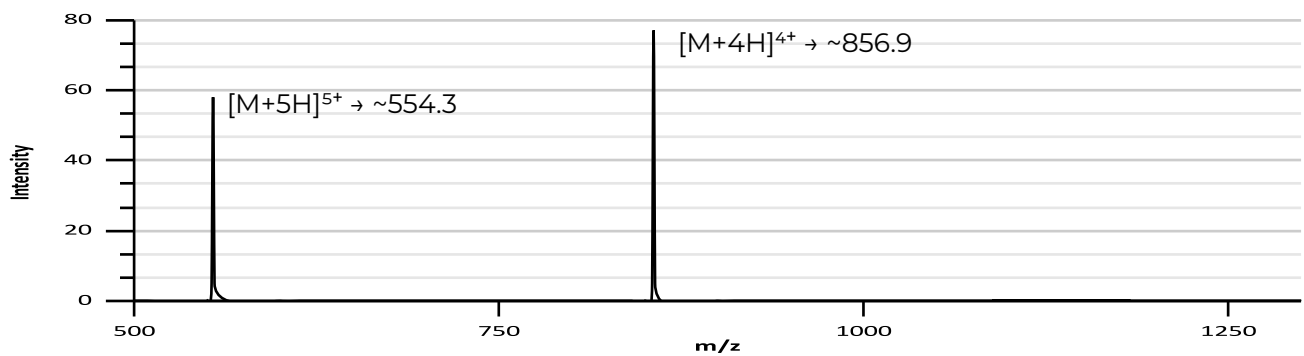
HPLC Chromatogram
