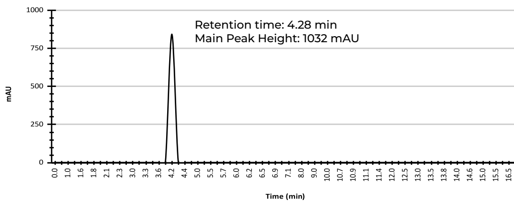
HPLC Chromatogram
