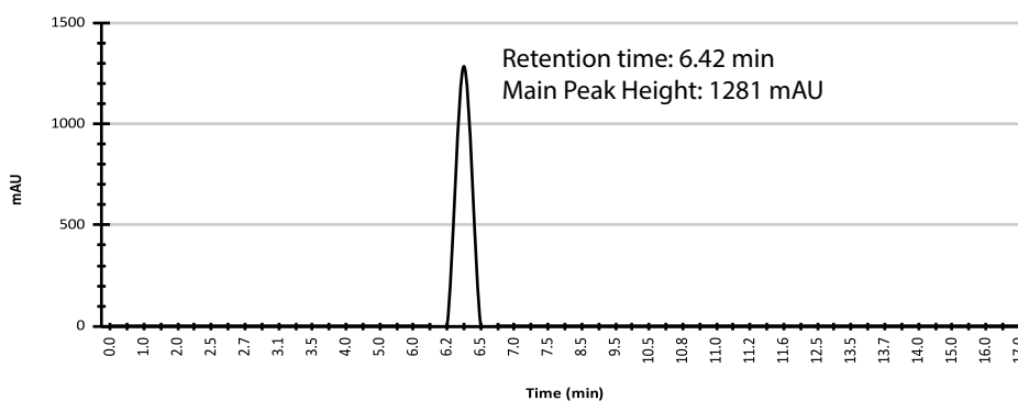
HPLC Chromatogram
