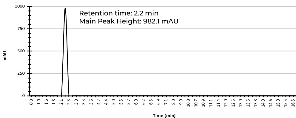
HPLC Chromatogram
