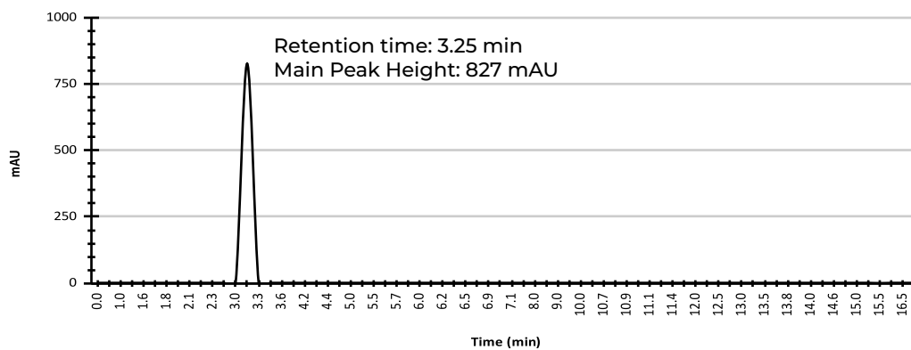
HPLC Chromatogram
