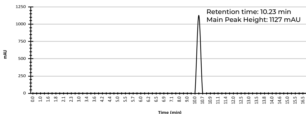
HPLC Chromatogram
