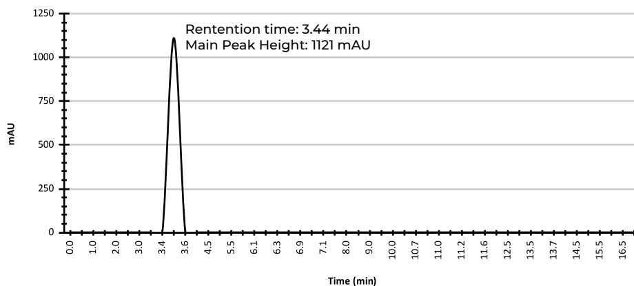
HPLC Chromatogram
