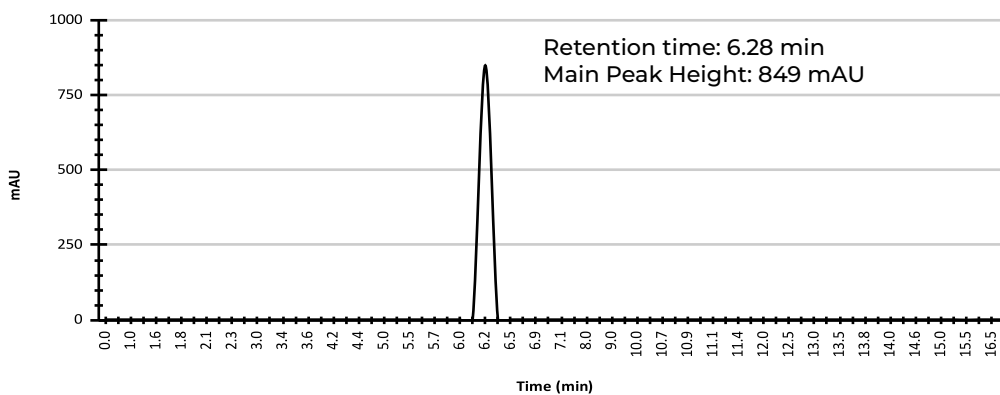
HPLC Chromatogram
