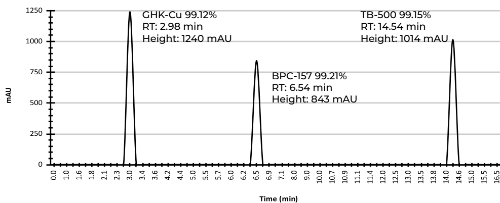
HPLC Chromatogram
