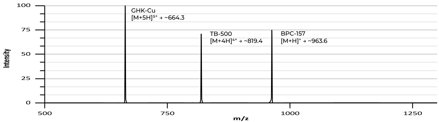
HPLC Chromatogram
