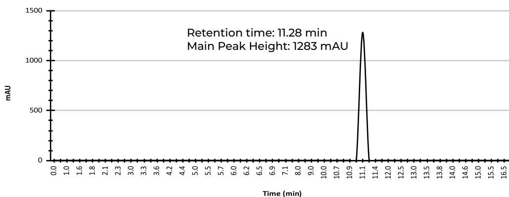
HPLC Chromatogram
