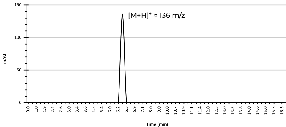
HPLC Chromatogram
