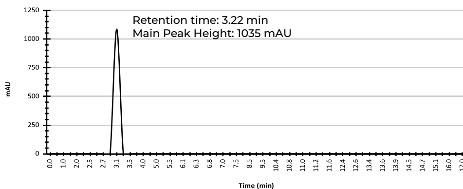
HPLC Chromatogram
