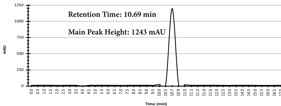
HPLC Chromatogram
