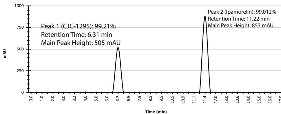
HPLC Chromatogram
