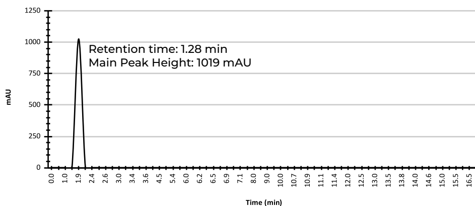
HPLC Chromatogram
